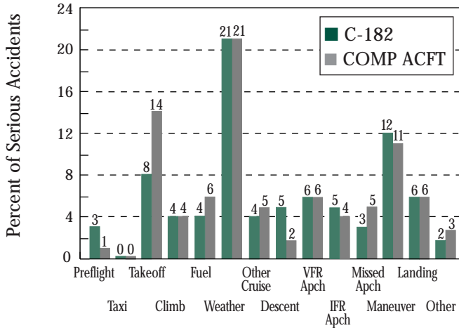
Figure 4. Pilot Related Causes Serious Accidents C-182
