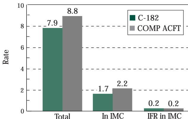
Figure 6. Night Accidents Per 100,000 Night Hours C-182
